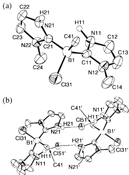
Fig. 1 An ORTEP 5 drawing of \{H_2[ClMeB(Im^{N-Me})_2]\}Cl \cdot C_6H_5Me ( \{H_2[2]\}Cl \cdot C_6H_5Me ) drawn at 50% probability level. All hydrogen atoms except those attached on the nitrogen atoms of the imidazolyl groups and the toluene molecule are omitted for clarity. (a) Cation part of the molecule ( i.e. \{H_2[2]\}^+ ). (b) Dimerized structure of \{H_2[2]\}Cl via intermolecular hydrogen bonding interaction.
