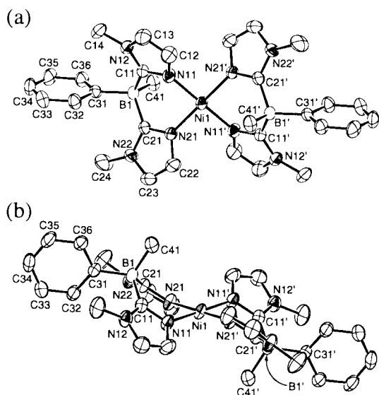
Fig. 3 An ORTEP diagram of \text{Ni}[\kappa^2\text{-MePhB}(\text{Im}^{N\text{-Me}})_2] ( \text{Ni}[4]_2 ) (50% probability level; all hydrogen atoms are omitted). (a) Perspective view. (b) 90^\circ rotated view of (a).
